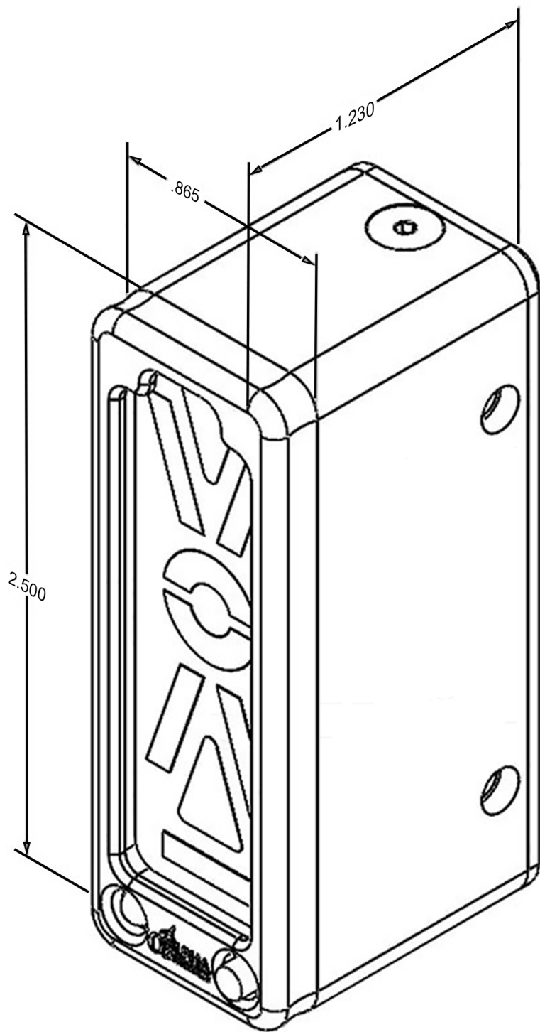
Eagle Display Technical Drawings With Dimensions
