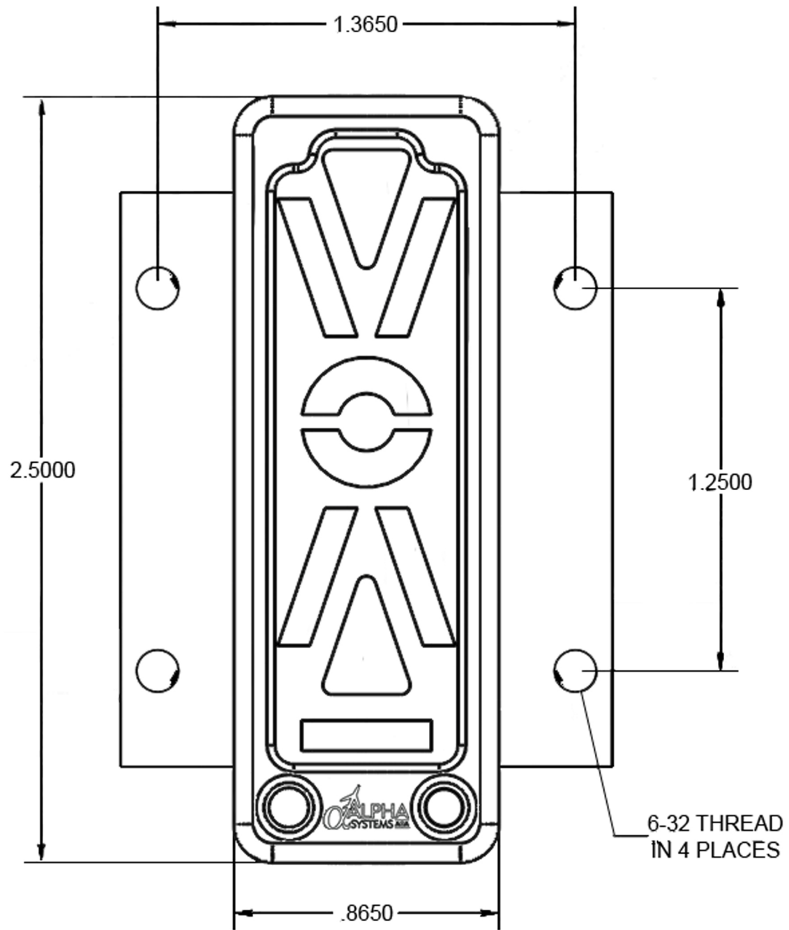
Eagle Display Technical Drawings With Dimensions
